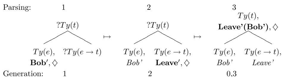
Figure 1: Parallel parsing and generation in DS
